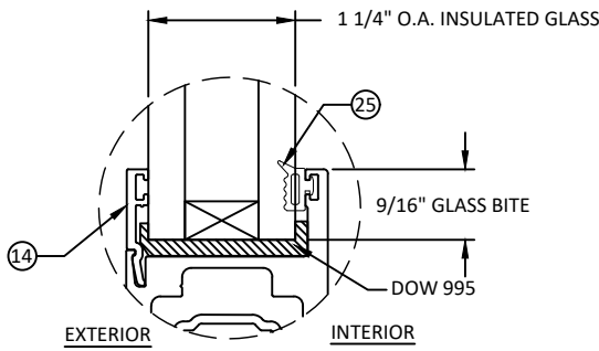
GLAZING DETAIL 2
