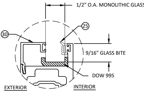
GLAZING DETAIL 1
